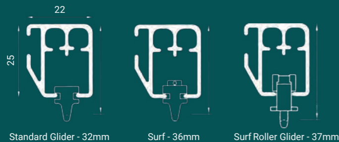
Standard Glider - 32mm Surf - 36mm Surf Roller Glider - 37mm
