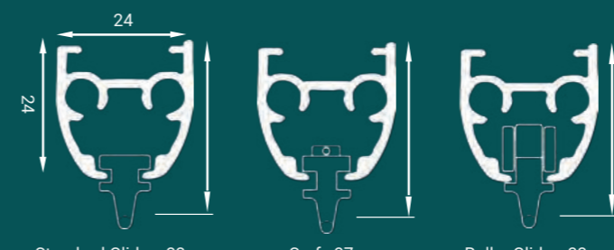
Standard Glider - 33mm Surf - 37mm Roller Glider - 33mm Surf Roller Glider - 38mm
